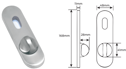
504AH - External plate with emergency release *
