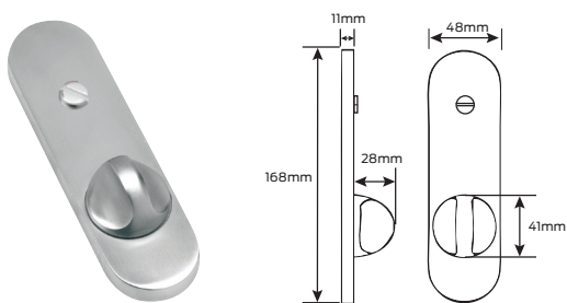
503AH - External plain plate
