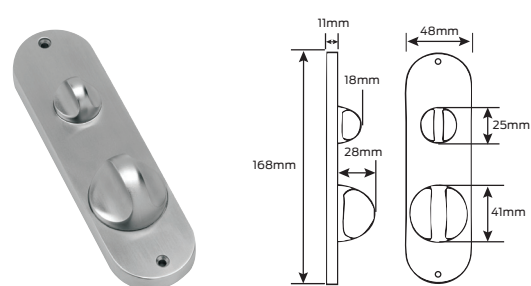
512AH - Internal plain plate
