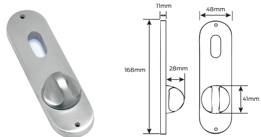
514AH - Internal plate with turn
